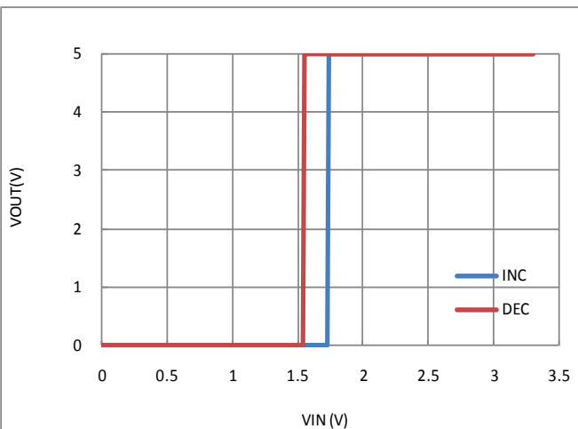
Figure 7 VOUT vs VIN (VCC=3.3V, VM=5V)
