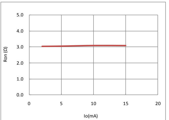
Figure 8 PI on Resistance vs Output Current (VCC=3.3V, VM=5V)
